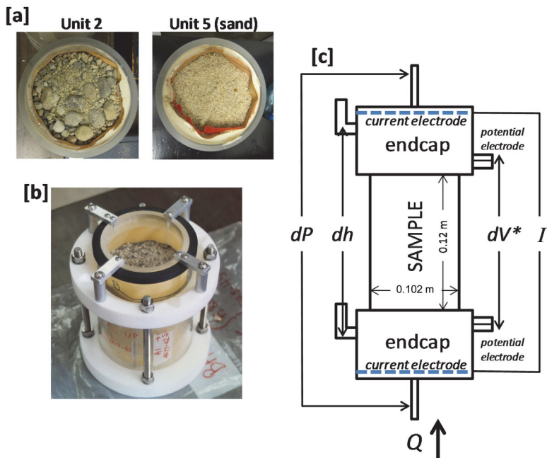
Figure 4. (a) Photos showing examples of reconstituted samples prepared in mould; (b) flexible sample holder used to prepare the samples; (c) schematic of the apparatus utilized for the joint measurement of hydraulic conductivity and complex conductivity ( dP = pressure gradient driving flow, dh = head drop across sample for Darcy calculation, dV^* = complex voltage recorded in response to current flow ( I )).
