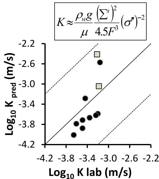
Figure 12. Predicted hydraulic conductivity from the Revil and Florsch [2010] model versus hydraulic conductivity measured using Darcy lab tests when imaginary conductivity is directly used for K estimation. The specific surface conductance of the Stern Layer ( \Sigma_s^s ) is assumed to equal 4\text{E-}09\text{S} ( \bar{\sigma}_d = 0.4 , AIC = -12.47 ). The 1:1 line (solid line) and the lines for \bar{\sigma}_d = \pm 1 (dashed lines) are shown to guide the eyes. Gray squares represent matrix only samples, whereas black circles are samples containing a cobble framework.
